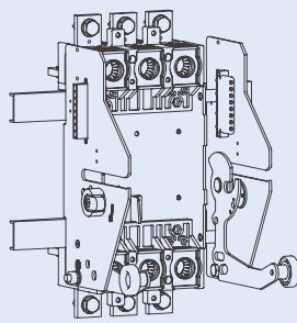
DIN-rail mounting
