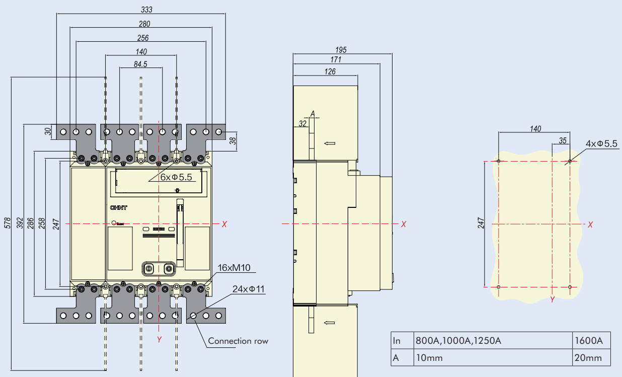
NM8N-1600 Front connection (Motor type 4P)
