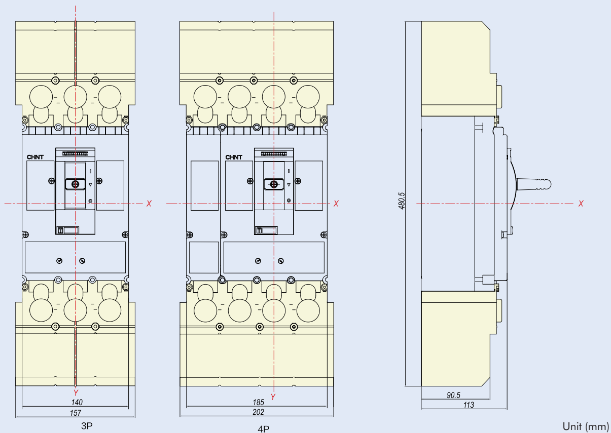
NM8N-400/630 Long terminal cover
