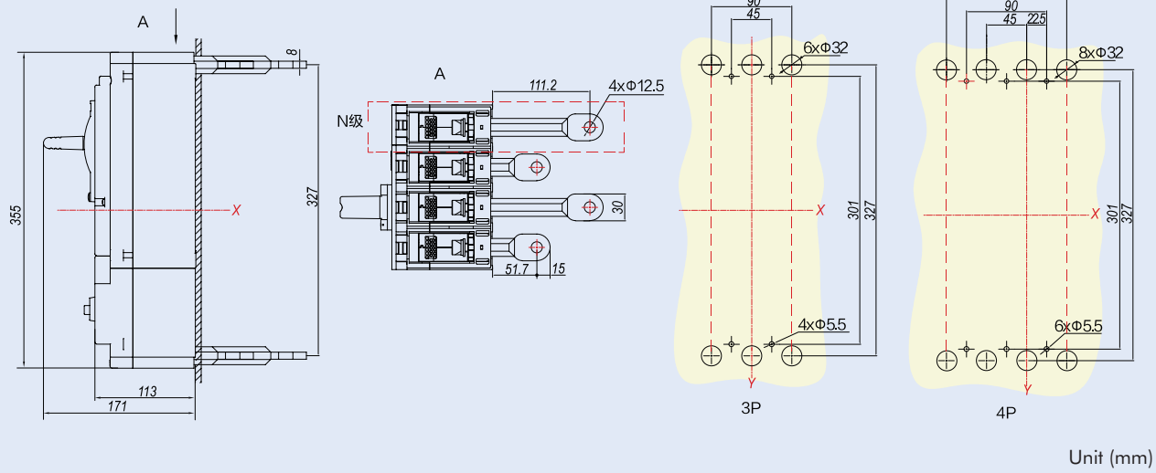
NM8NL-400/630 Rear connection
