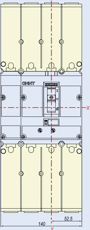
4P Long terminal cover
