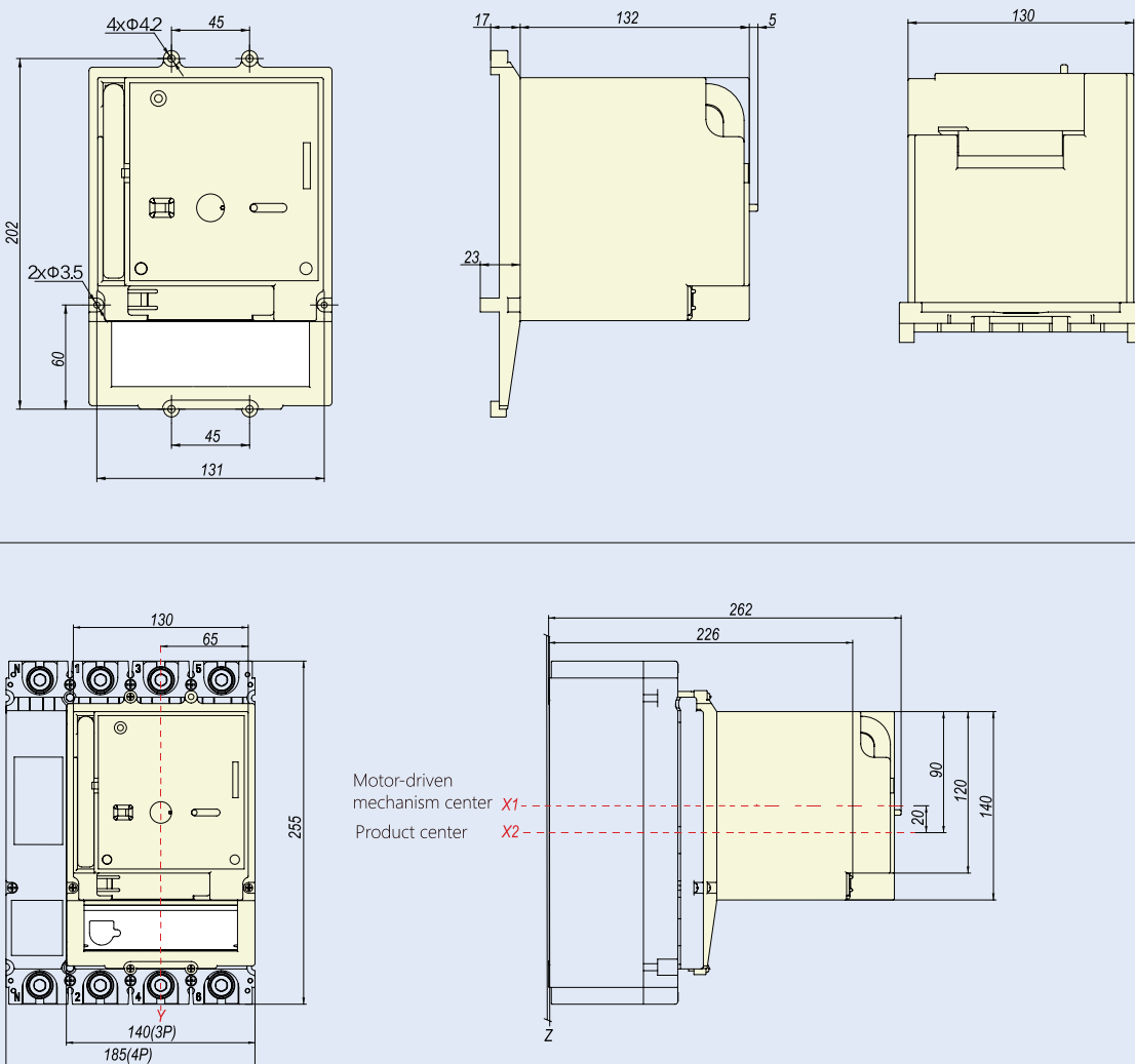
Overall and mounting dimension of MOD23-M8
