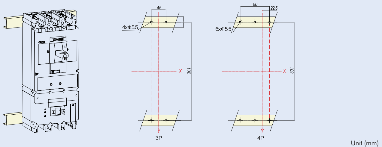
NM8NL-400/630 DIN-rail mounting
