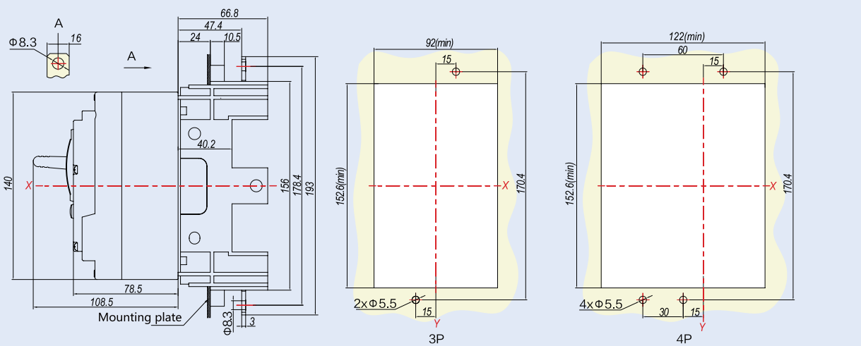
NM8N-125 Plug-in front connection
