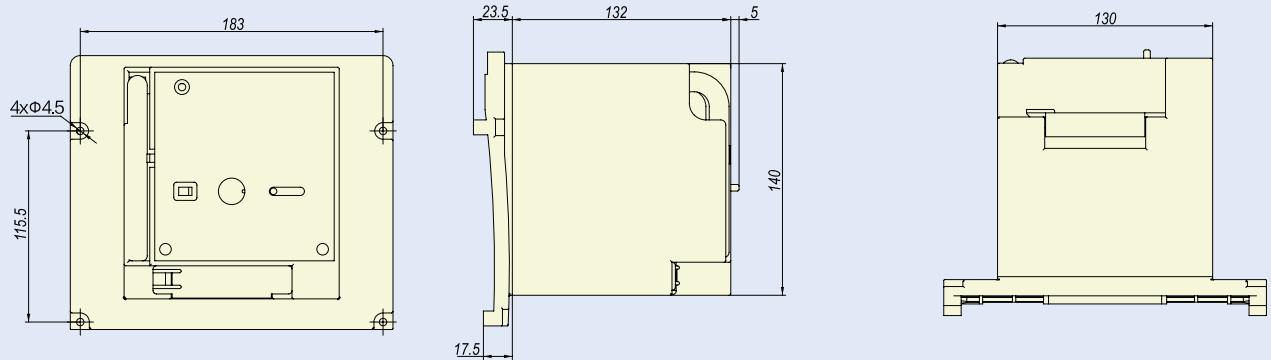
Overall and mounting dimension of MOD24-M8
