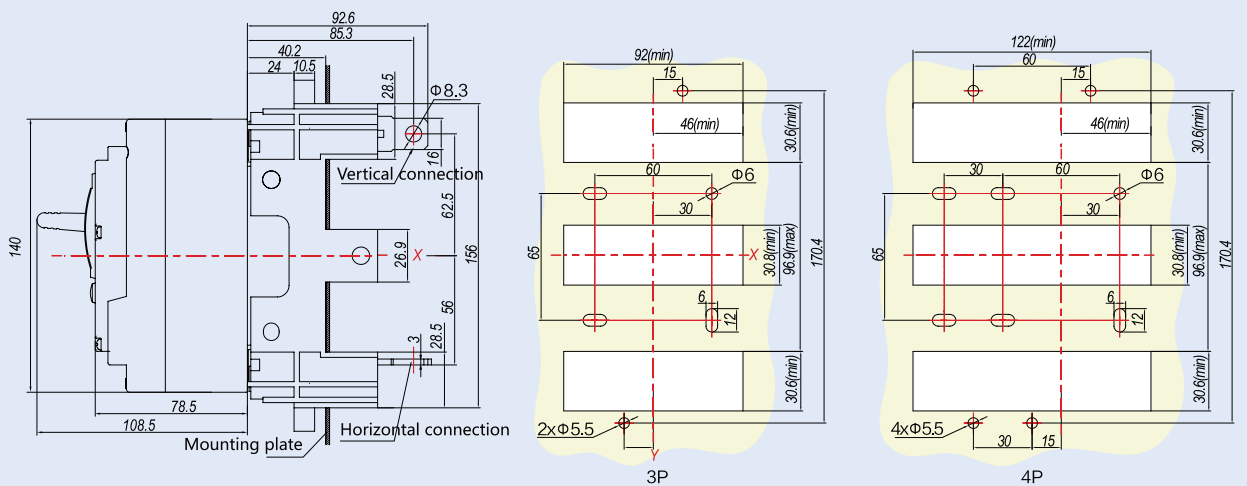
NM8N-125 Plug-in rear connection
