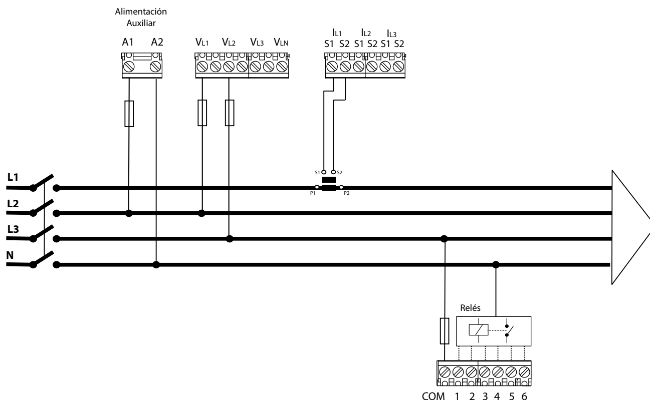
Figura 7: 2 tensiones y 1 corriente, modelo Controller MASTER control VAR 6.
