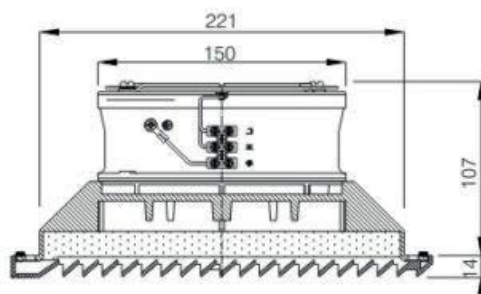
Outline Dimensions (Units:mm)
