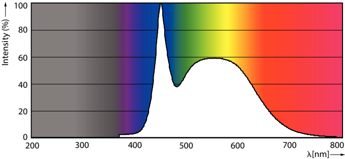
Spectral Power Distribution Colour - EcoHome LEDBulb 9W E27 6500KHV 1PF/20AR
