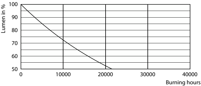
Lumen Maintenance Diagram - EcoHome LEDBulb 9W E27 6500KHV 1PF/20AR
