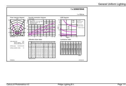
General uniform lighting - EcoHome LEDBulb 9W E27 6500KHV 1PF/20AR
