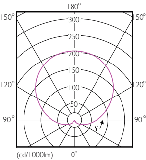
Light Distribution Diagram - EcoHome LEDBulb 9W E27 6500KHV 1PF/20AR
