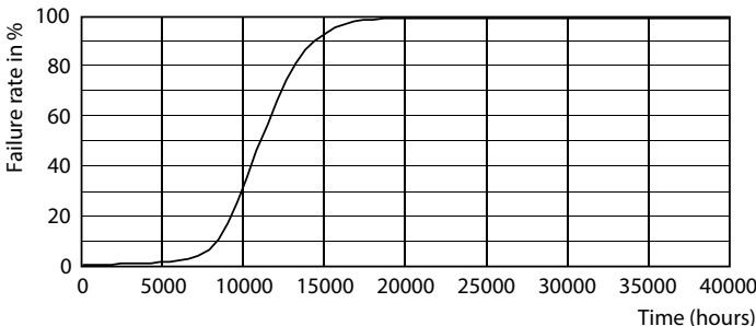
Life Expectancy Diagram - EcoHome LEDBulb 9W E27 6500KHV 1PF/20AR
